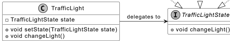
State design pattern
