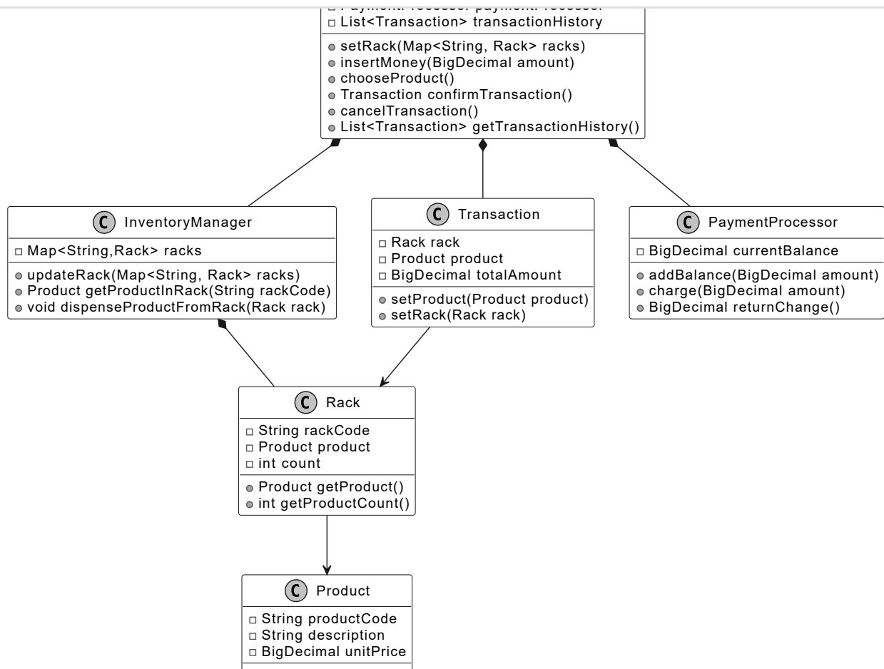
Class Diagram of Vending Machine
